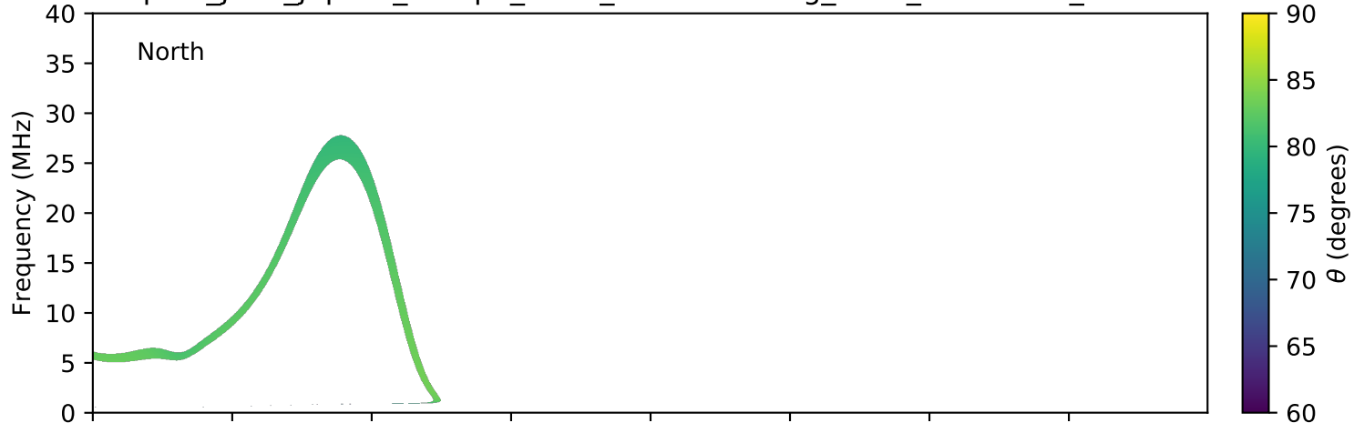
expres_juno_jupiter_europa_isaac_lossc-wid1deg_3kev_20180505_v01.cdf
