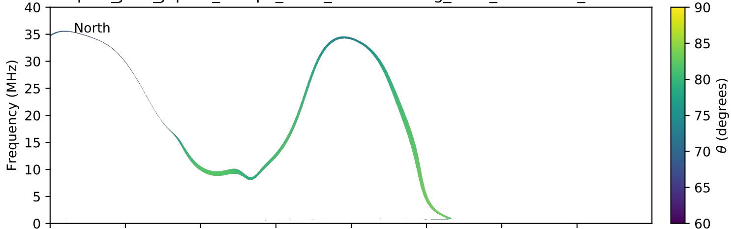
expres_juno_jupiter_europa_isaac_lossc-wid1deg_3kev_20180501_v01.cdf
