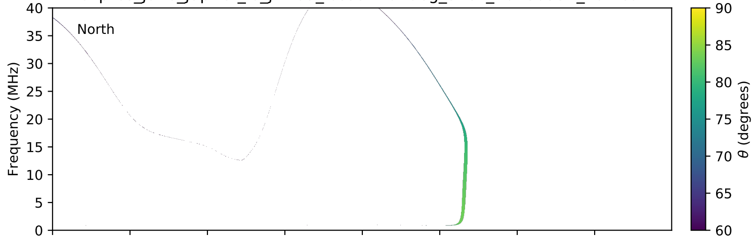
expres_juno_jupiter_io_jrm09_lossc-wid1deg_3kev_20180331_v01.cdf
