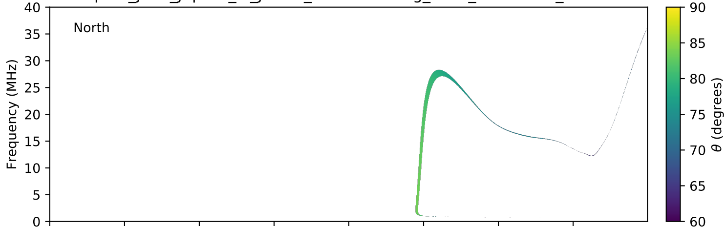
expres_juno_jupiter_io_jrm09_lossc-wid1deg_3kev_20180325_v01.cdf
