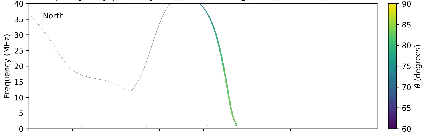
expres_juno_jupiter_io_jrm09_lossc-wid1deg_3kev_20180324_v01.cdf
