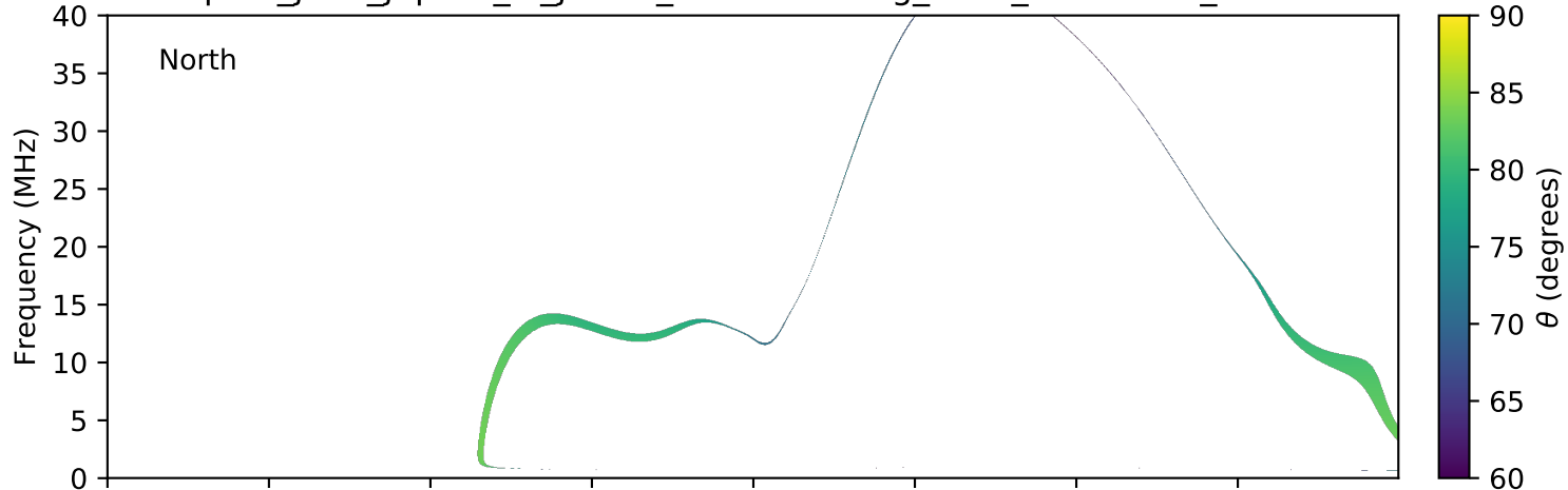
expres_juno_jupiter_io_jrm09_lossc-wid1deg_3kev_20180320_v01.cdf
