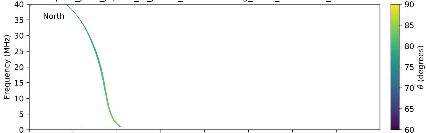
expres_juno_jupiter_io_jrm09_lossc-wid1deg_3kev_20180319_v01.cdf
