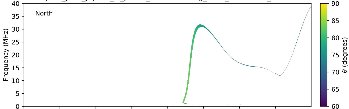
expres_juno_jupiter_io_jrm09_lossc-wid1deg_3kev_20180318_v01.cdf
