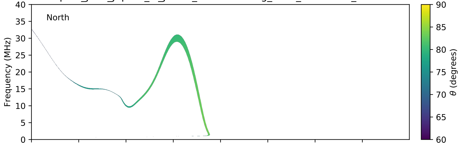
expres_juno_jupiter_io_jrm09_lossc-wid1deg_3kev_20180310_v01.cdf
