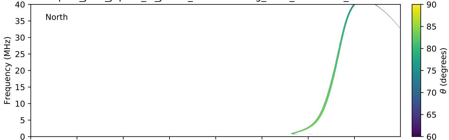
expres_juno_jupiter_io_jrm09_lossc-wid1deg_3kev_20180309_v01.cdf
