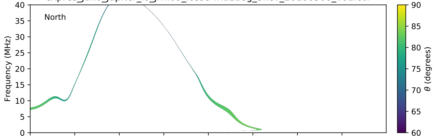
expres_juno_jupiter_io_jrm09_lossc-wid1deg_3kev_20180308_v01.cdf
