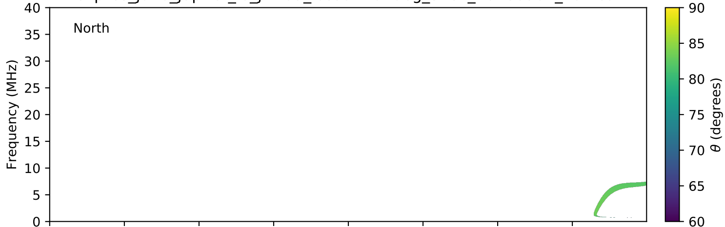
expres_juno_jupiter_io_jrm09_lossc-wid1deg_3kev_20180307_v01.cdf
