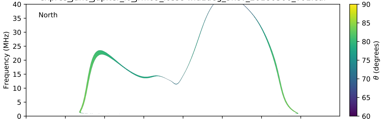
expres_juno_jupiter_io_jrm09_lossc-wid1deg_3kev_20180306_v01.cdf
