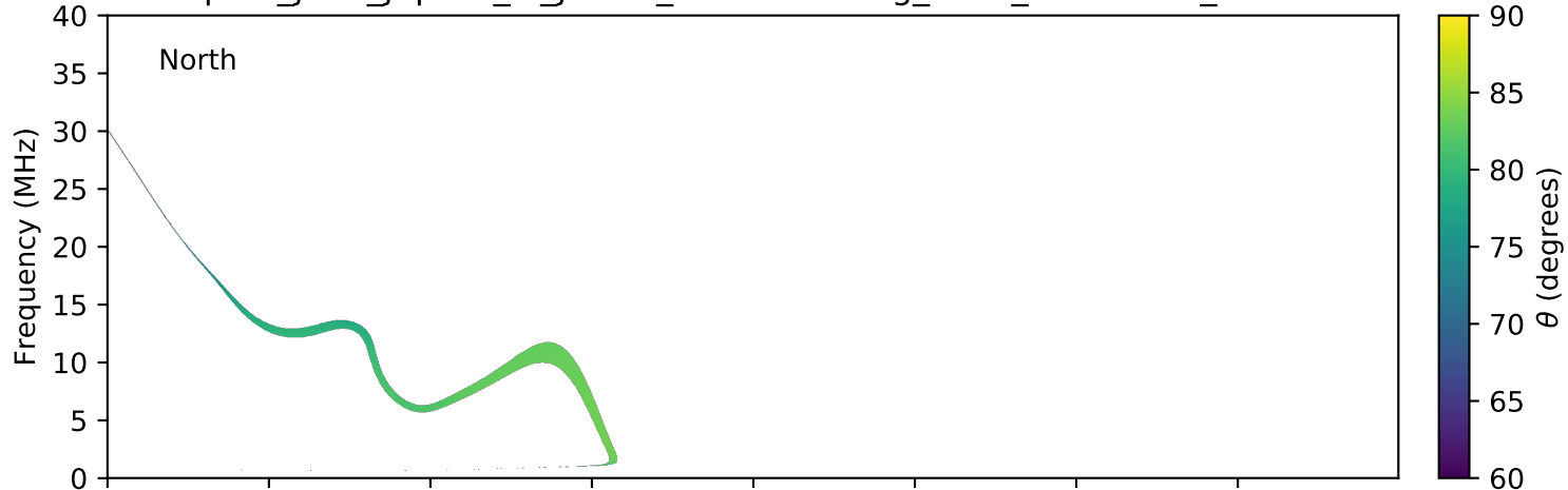
expres_juno_jupiter_io_jrm09_lossc-wid1deg_3kev_20180303_v01.cdf
