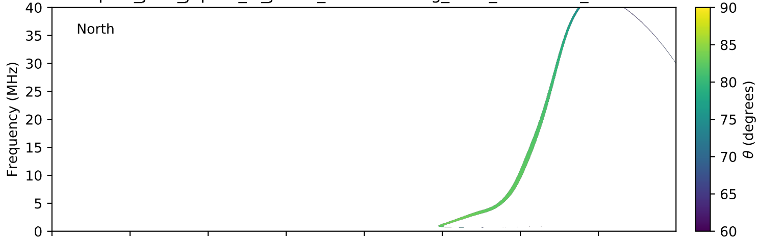
expres_juno_jupiter_io_jrm09_lossc-wid1deg_3kev_20180302_v01.cdf
