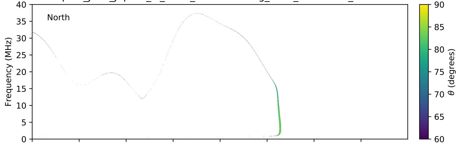
expres_juno_jupiter_io_isaac_lossc-wid1deg_3kev_20180331_v01.cdf
