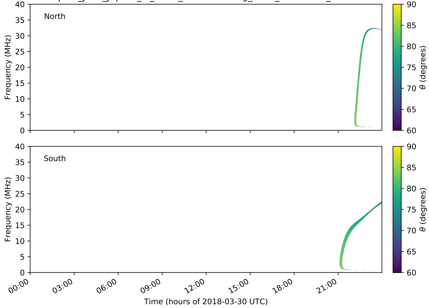
expres_juno_jupiter_io_isaac_lossc-wid1deg_3kev_20180330_v01.cdf
