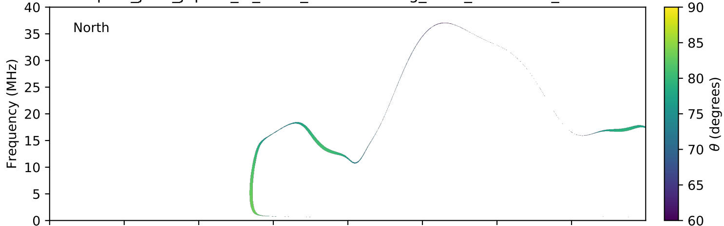
expres_juno_jupiter_io_isaac_lossc-wid1deg_3kev_20180327_v01.cdf
