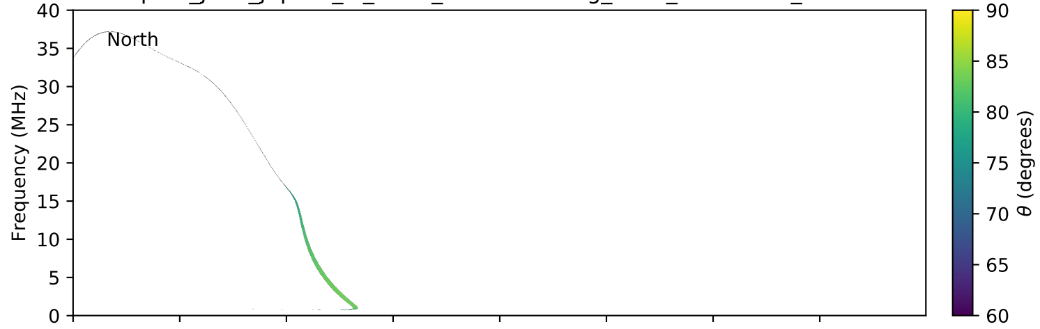
expres_juno_jupiter_io_isaac_lossc-wid1deg_3kev_20180326_v01.cdf
