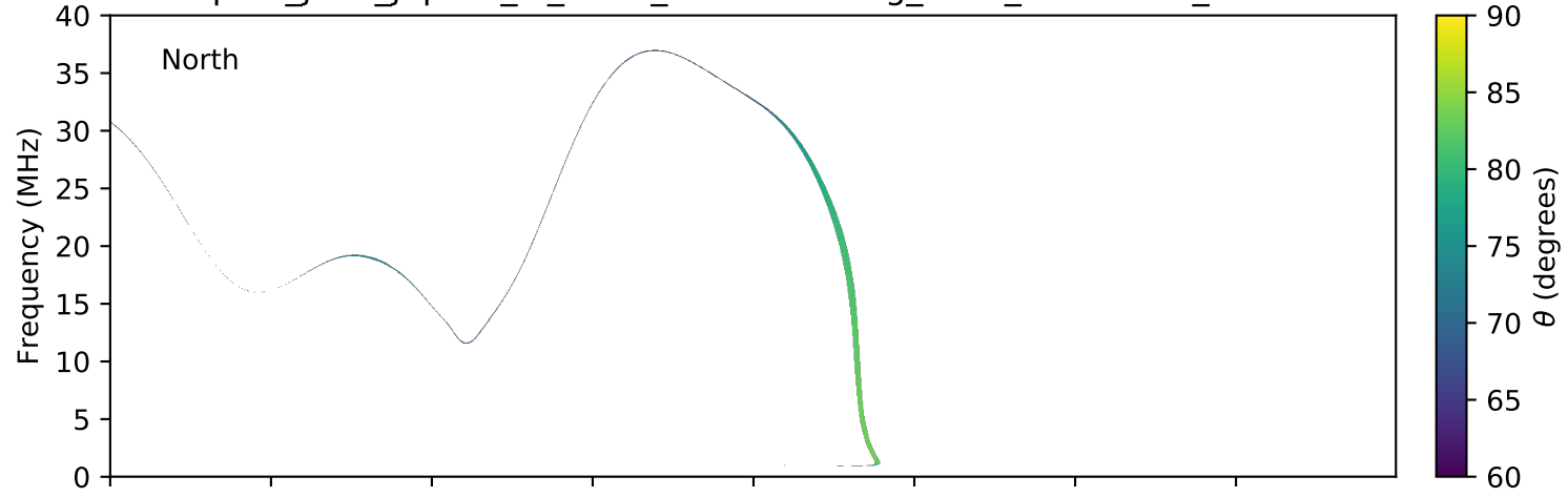
expres_juno_jupiter_io_isaac_lossc-wid1deg_3kev_20180324_v01.cdf
