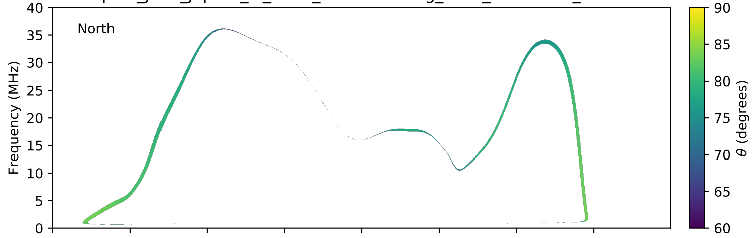
expres_juno_jupiter_io_isaac_lossc-wid1deg_3kev_20180322_v01.cdf
