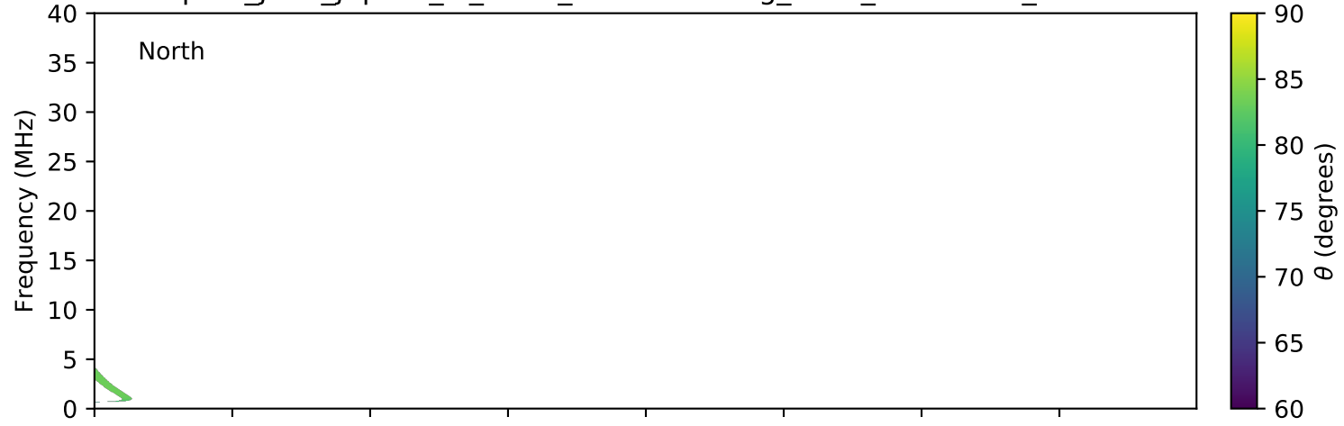
expres_juno_jupiter_io_isaac_lossc-wid1deg_3kev_20180321_v01.cdf
