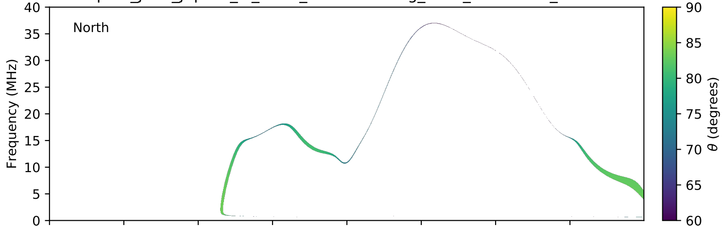
expres_juno_jupiter_io_isaac_lossc-wid1deg_3kev_20180320_v01.cdf
