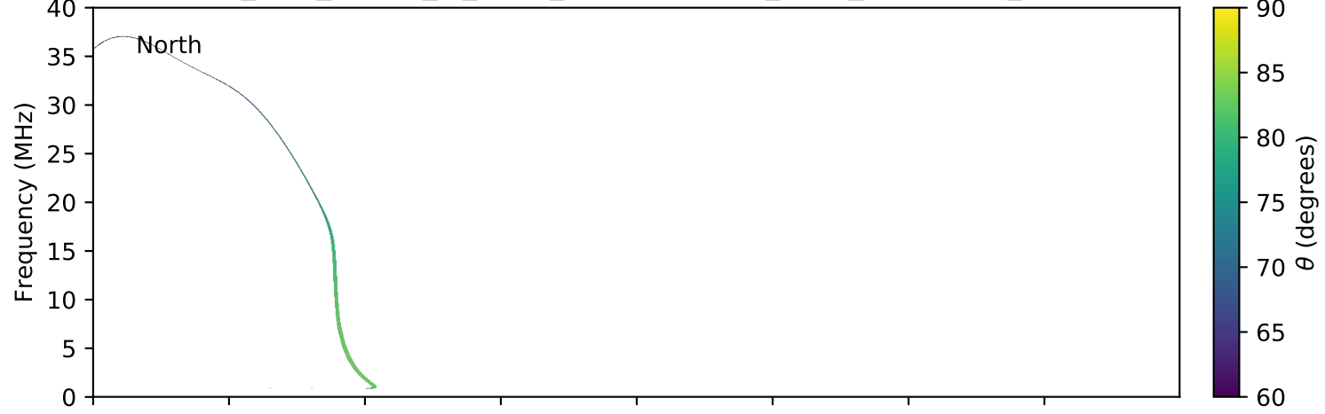
expres_juno_jupiter_io_isaac_lossc-wid1deg_3kev_20180319_v01.cdf
