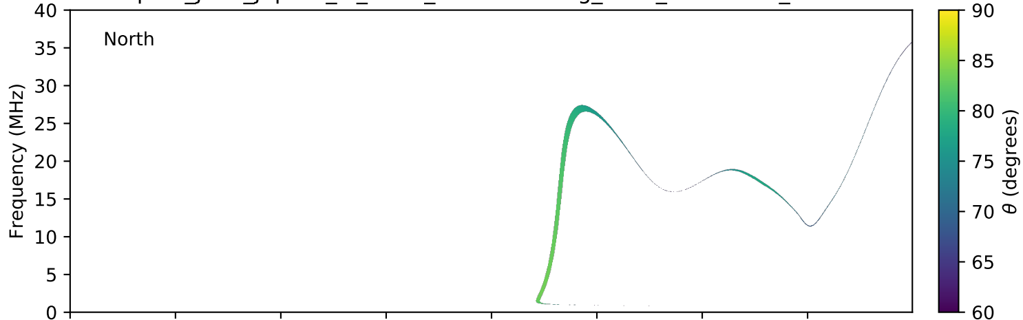
expres_juno_jupiter_io_isaac_lossc-wid1deg_3kev_20180318_v01.cdf
