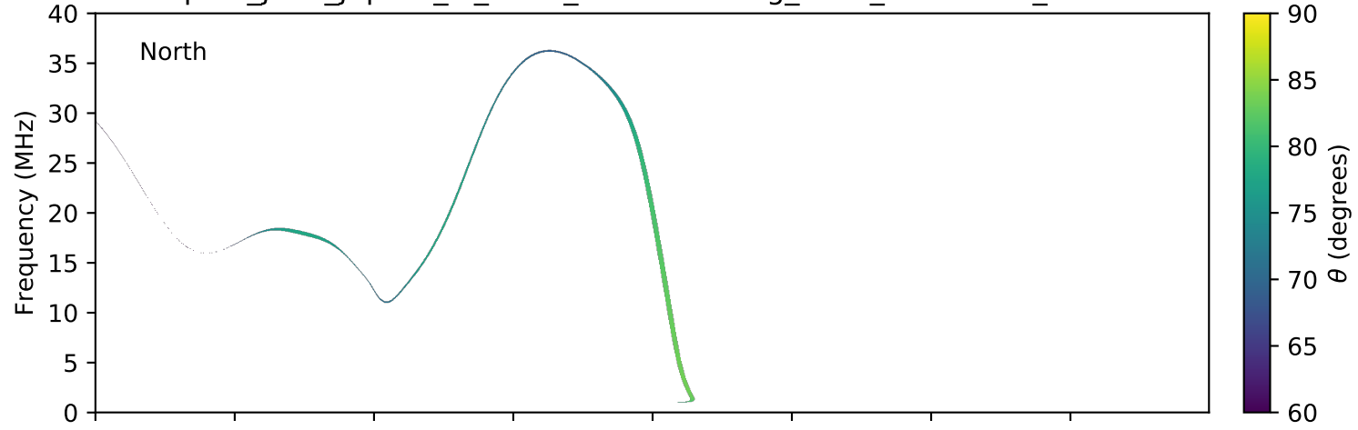
expres_juno_jupiter_io_isaac_lossc-wid1deg_3kev_20180317_v01.cdf
