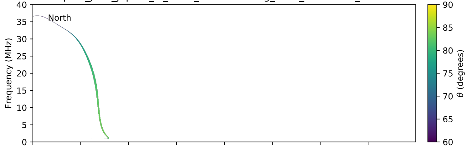
expres_juno_jupiter_io_isaac_lossc-wid1deg_3kev_20180312_v01.cdf
