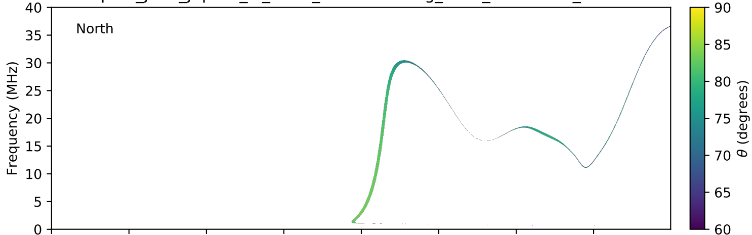
expres_juno_jupiter_io_isaac_lossc-wid1deg_3kev_20180311_v01.cdf
