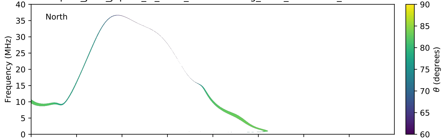
expres_juno_jupiter_io_isaac_lossc-wid1deg_3kev_20180308_v01.cdf
