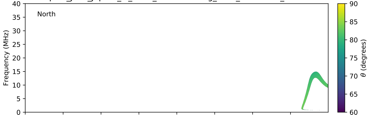
expres_juno_jupiter_io_isaac_lossc-wid1deg_3kev_20180307_v01.cdf
