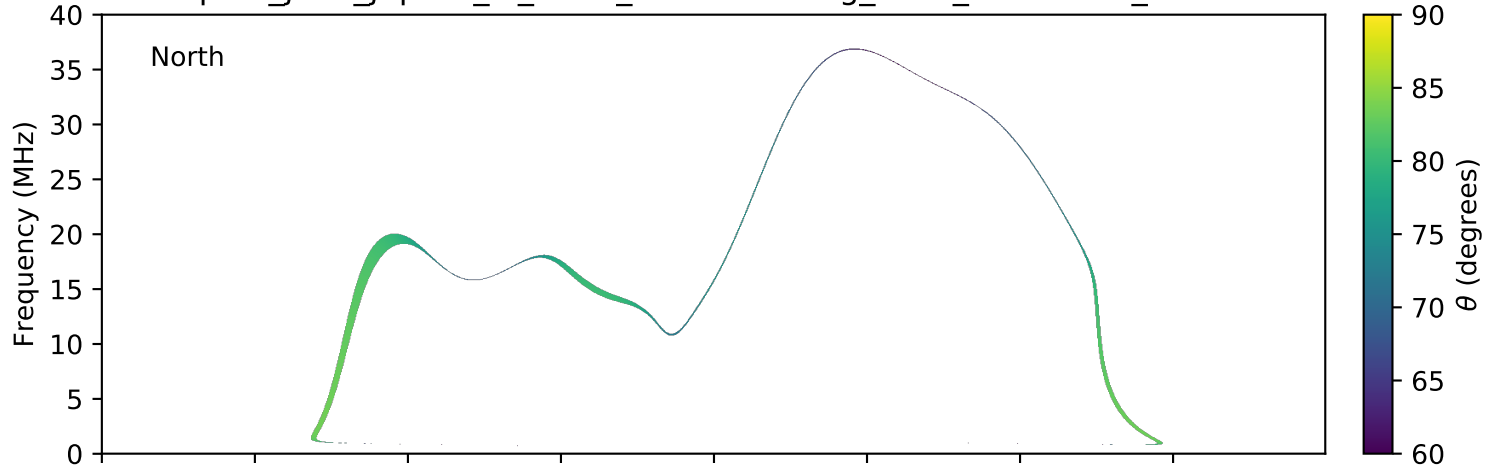
expres_juno_jupiter_io_isaac_lossc-wid1deg_3kev_20180306_v01.cdf
