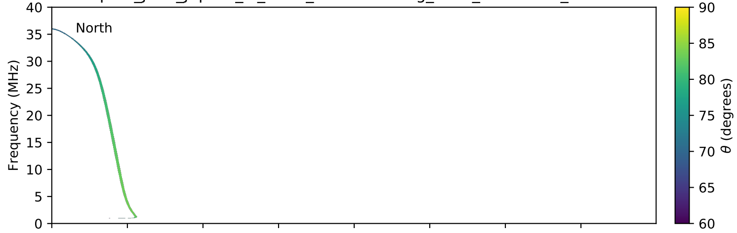
expres_juno_jupiter_io_isaac_lossc-wid1deg_3kev_20180305_v01.cdf
