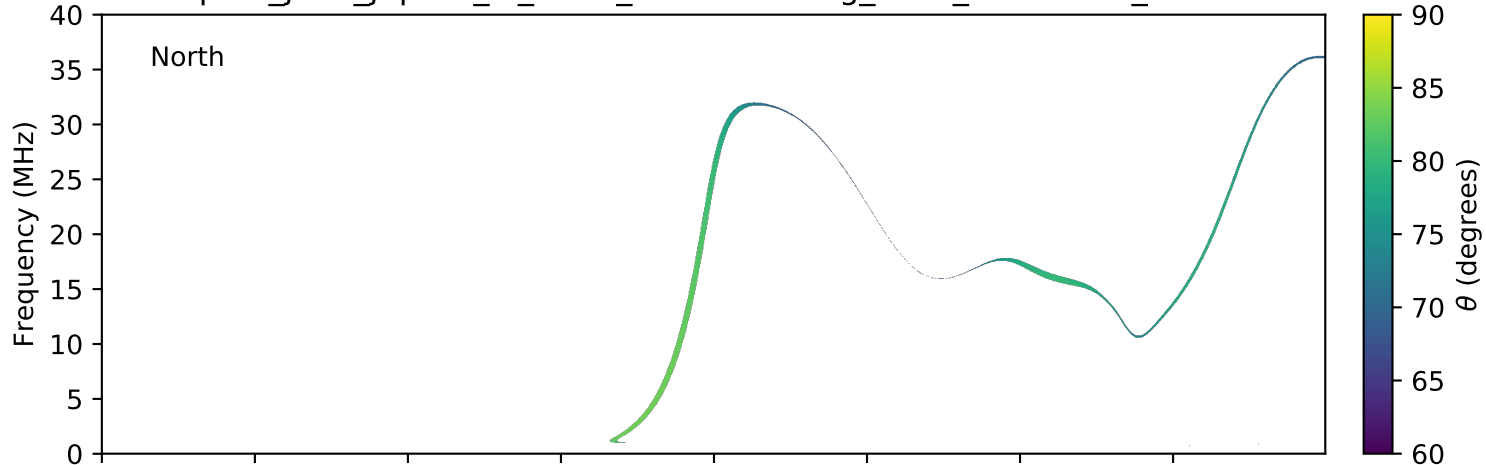
expres_juno_jupiter_io_isaac_lossc-wid1deg_3kev_20180304_v01.cdf
