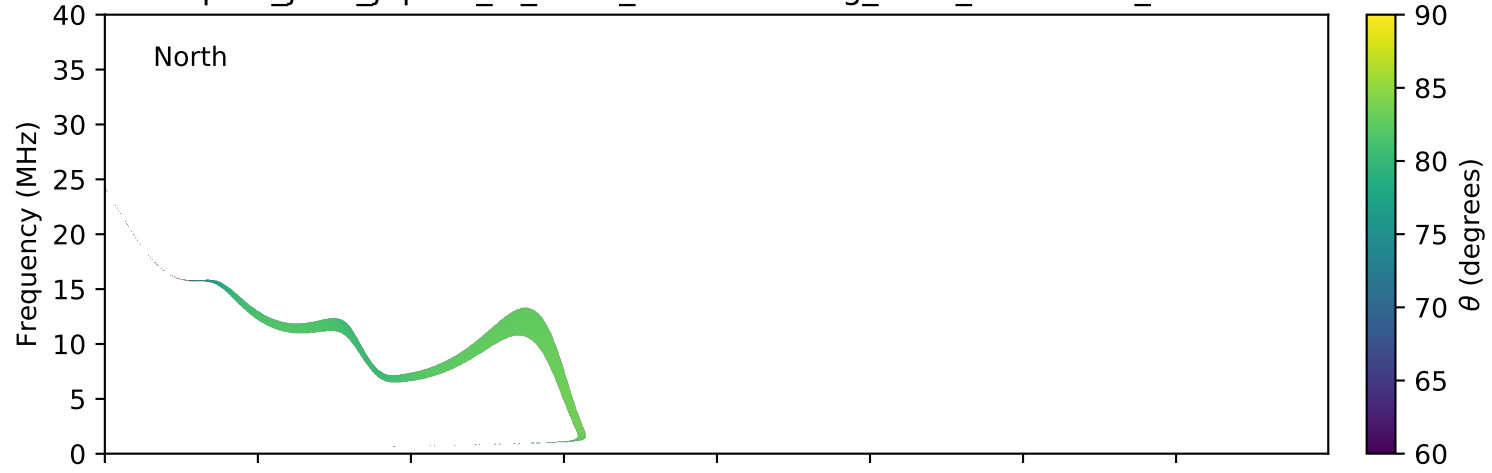
expres_juno_jupiter_io_isaac_lossc-wid1deg_3kev_20180303_v01.cdf
