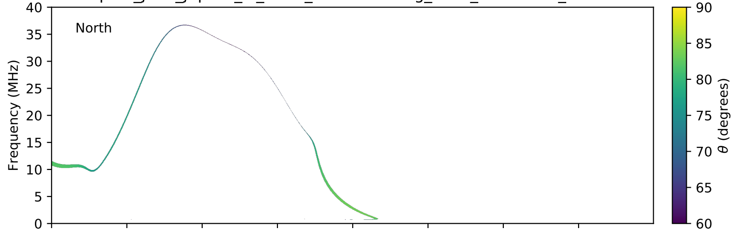
expres_juno_jupiter_io_isaac_lossc-wid1deg_3kev_20180301_v01.cdf
