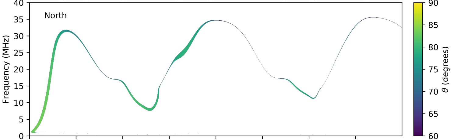
expres_juno_jupiter_ganymede_isaac_lossc-wid1deg_3kev_20180328_v01.cdf
