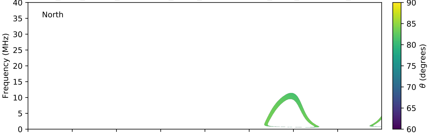
expres_juno_jupiter_ganymede_isaac_lossc-wid1deg_3kev_20180320_v01.cdf
