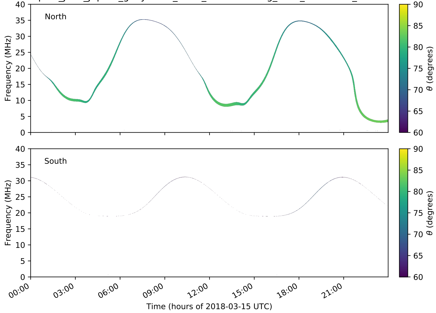
expres_juno_jupiter_ganymede_isaac_lossc-wid1deg_3kev_20180315_v01.cdf
