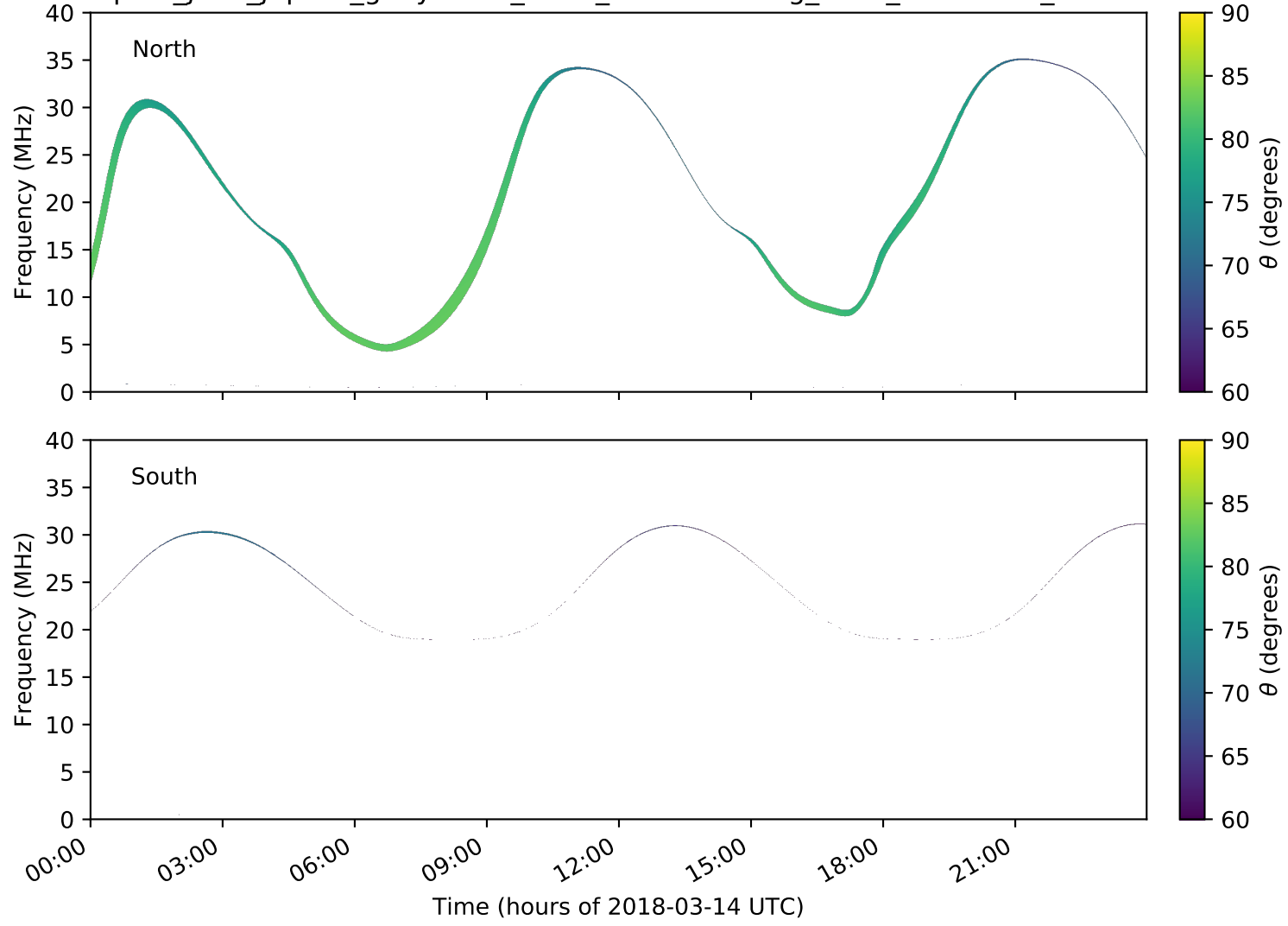
expres_juno_jupiter_ganymede_isaac_lossc-wid1deg_3kev_20180314_v01.cdf
