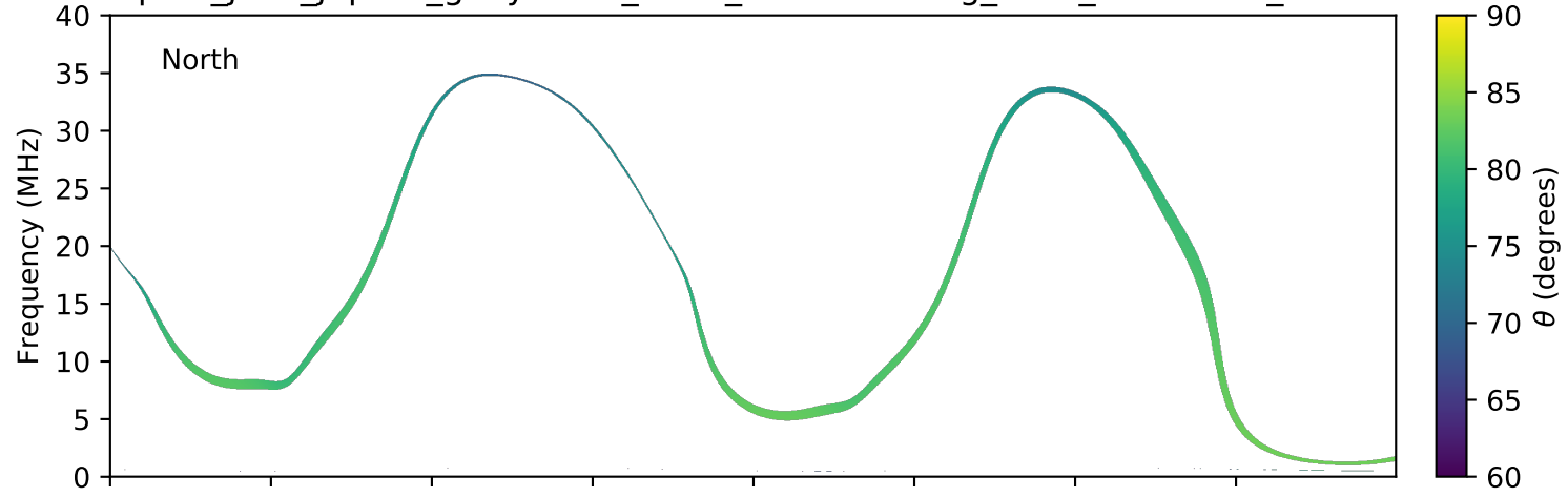
expres_juno_jupiter_ganymede_isaac_lossc-wid1deg_3kev_20180308_v01.cdf
