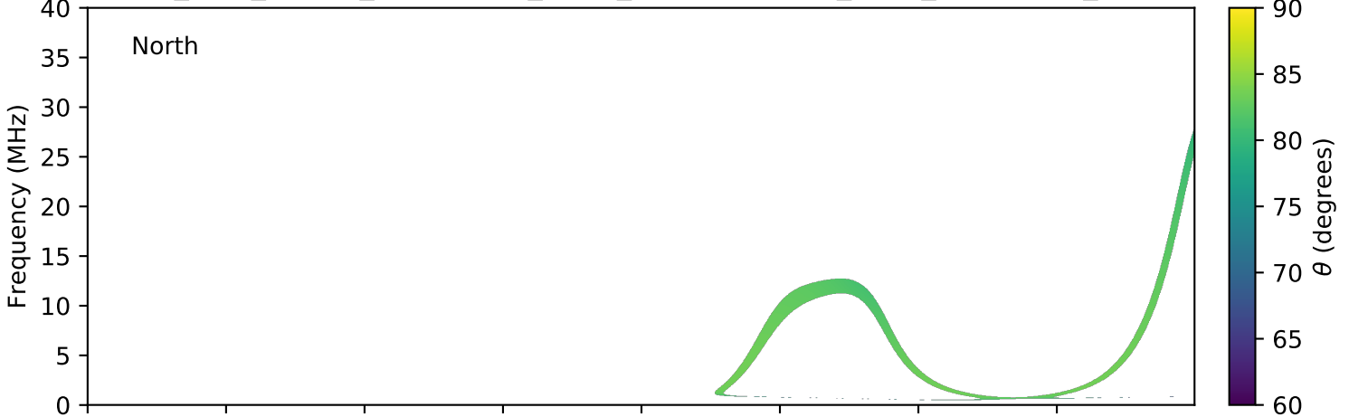
expres_juno_jupiter_ganymede_isaac_lossc-wid1deg_3kev_20180306_v01.cdf
