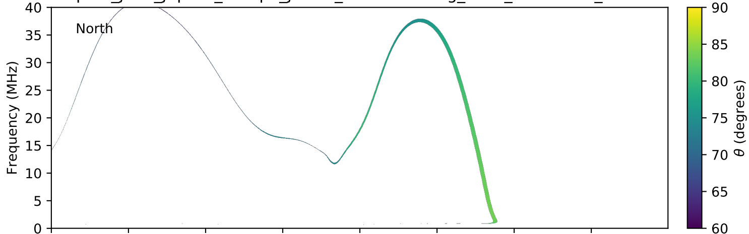
expres_juno_jupiter_europa_jrm09_lossc-wid1deg_3kev_20180328_v01.cdf
