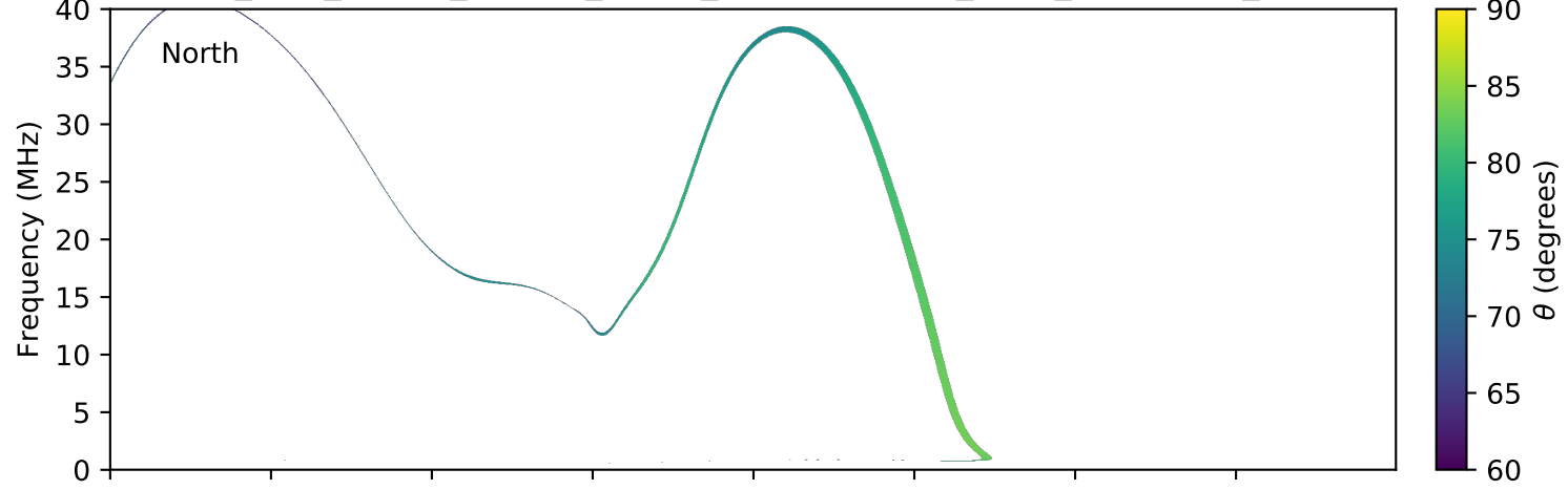
expres_juno_jupiter_europa_jrm09_lossc-wid1deg_3kev_20180326_v01.cdf
