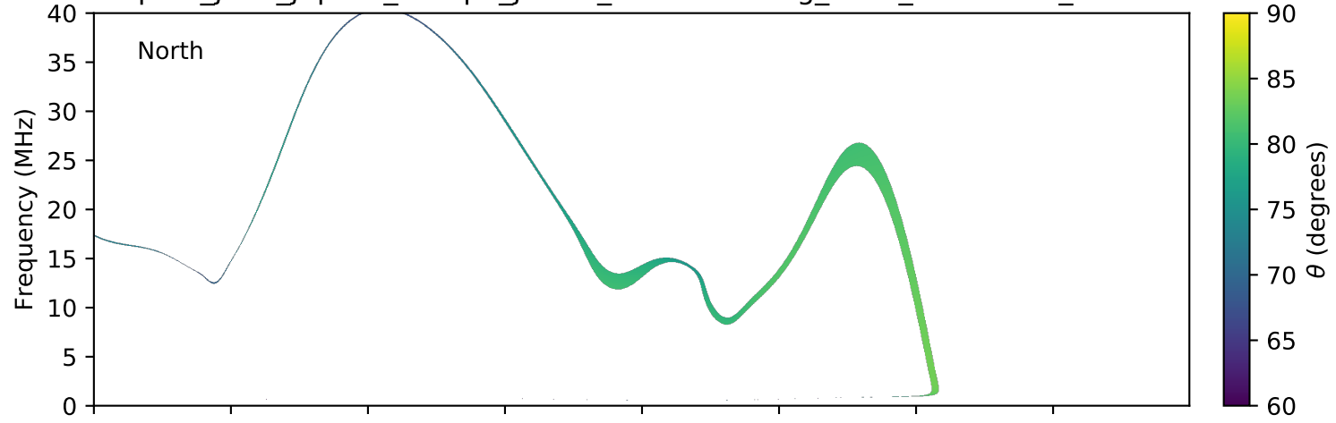
expres_juno_jupiter_europa_jrm09_lossc-wid1deg_3kev_20180325_v01.cdf
