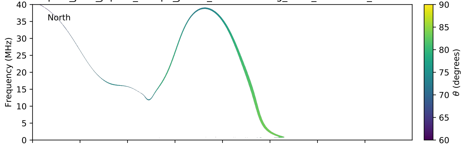
expres_juno_jupiter_europa_jrm09_lossc-wid1deg_3kev_20180324_v01.cdf
