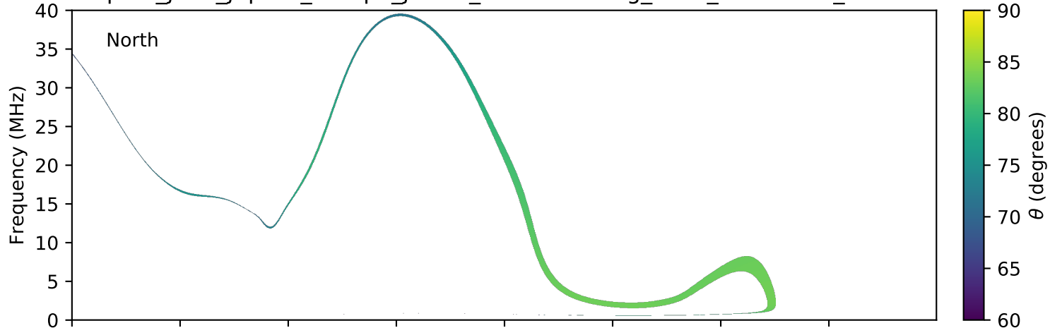
expres_juno_jupiter_europa_jrm09_lossc-wid1deg_3kev_20180322_v01.cdf
