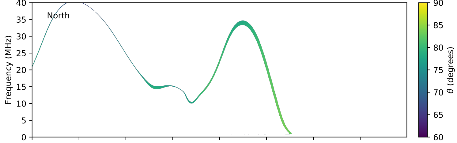
expres_juno_jupiter_europa_jrm09_lossc-wid1deg_3kev_20180321_v01.cdf
