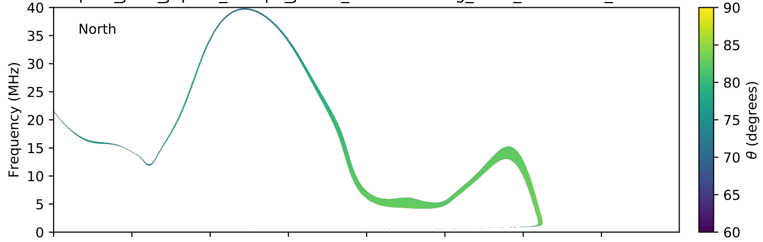
expres_juno_jupiter_europa_jrm09_lossc-wid1deg_3kev_20180320_v01.cdf
