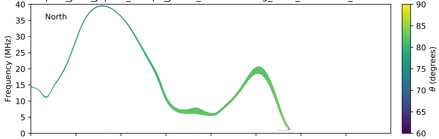
expres_juno_jupiter_europa_jrm09_lossc-wid1deg_3kev_20180311_v01.cdf
