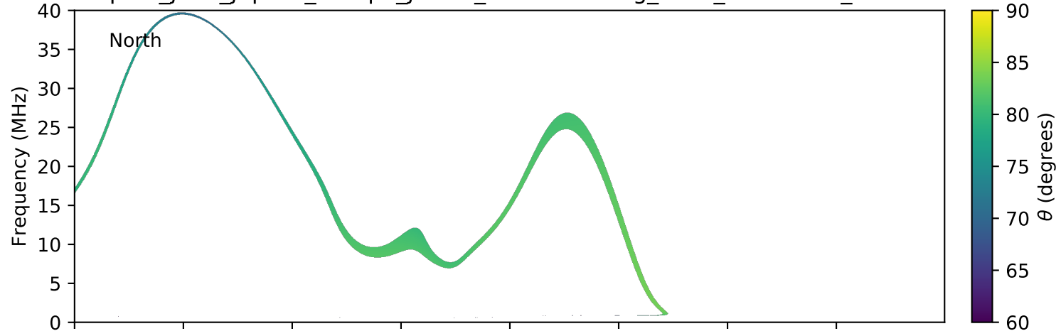
expres_juno_jupiter_europa_jrm09_lossc-wid1deg_3kev_20180309_v01.cdf
